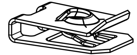
3D-Ansicht / isometrical view 2:1
